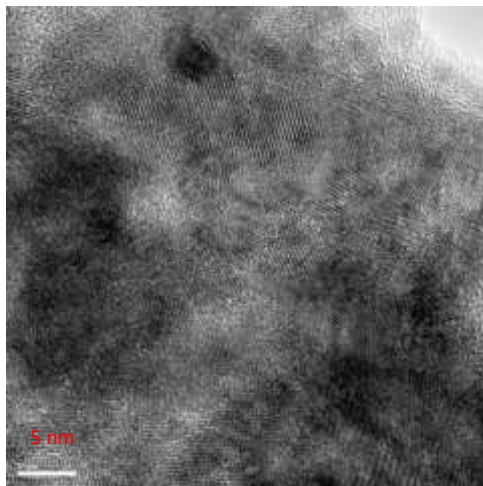
(a) smectite
