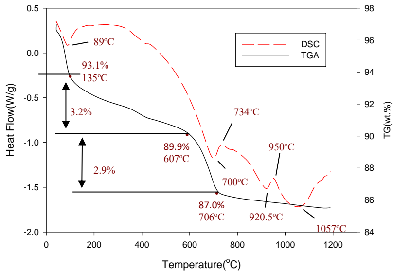
Figure 7. DSC and TGA analysis of the smectite (before being sintered at high temperatures)
