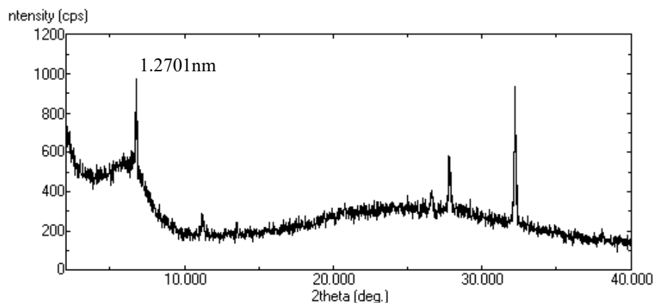
Figure 4. XRD analysis of the smectite-Ag/Zn (sintered at 350^\circ\text{C} )
