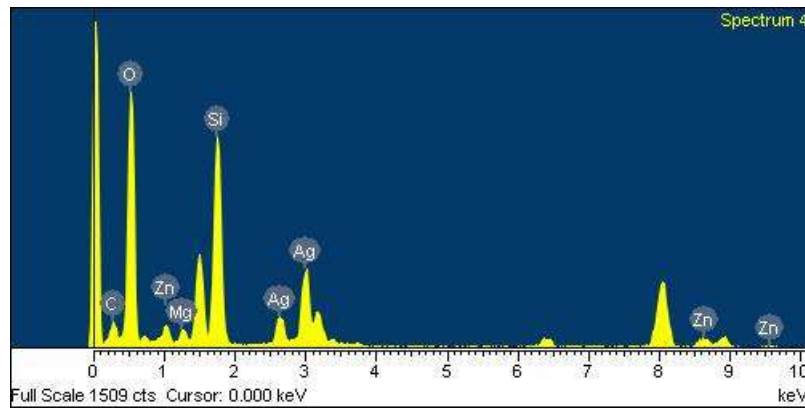
Figure 6. EDS analysis results of the smectite-Ag/Zn
