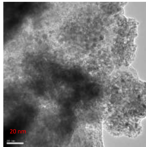
(b) smectite
