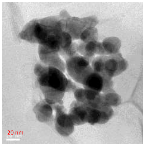
(c) smectite-Ag/Zn
