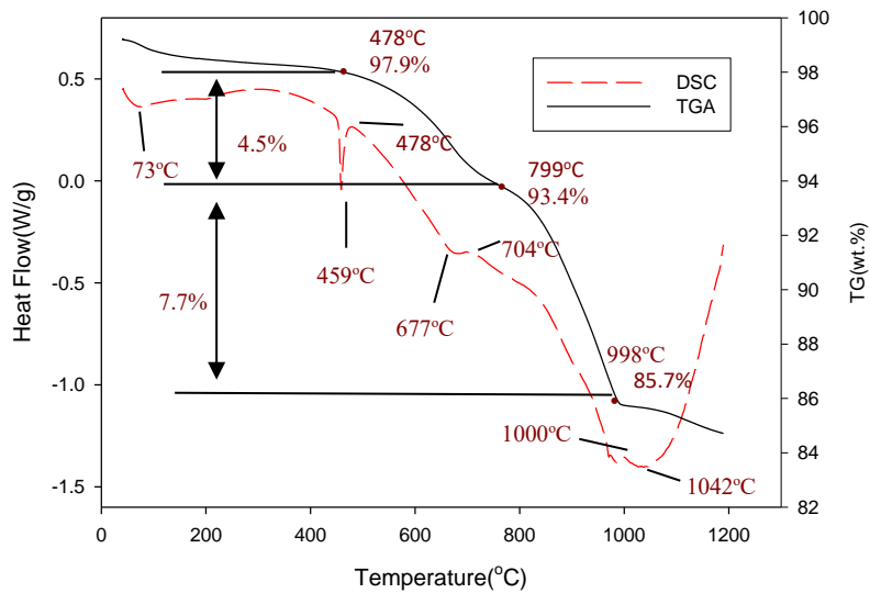
Figure 8. DSC and TGA analysis of the smectite-Ag/Zn
